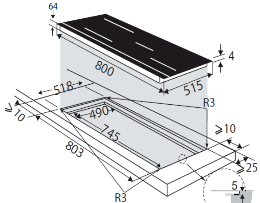
Fitting flush with the worktop
