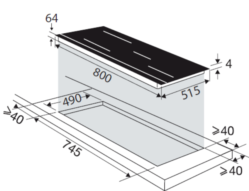
Fitting into the worktop
