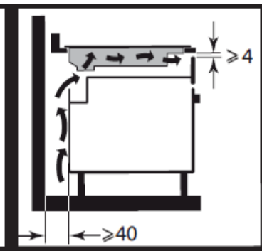
Fitting flush with the worktop
