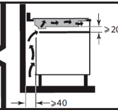
Fitting flush with the worktop
